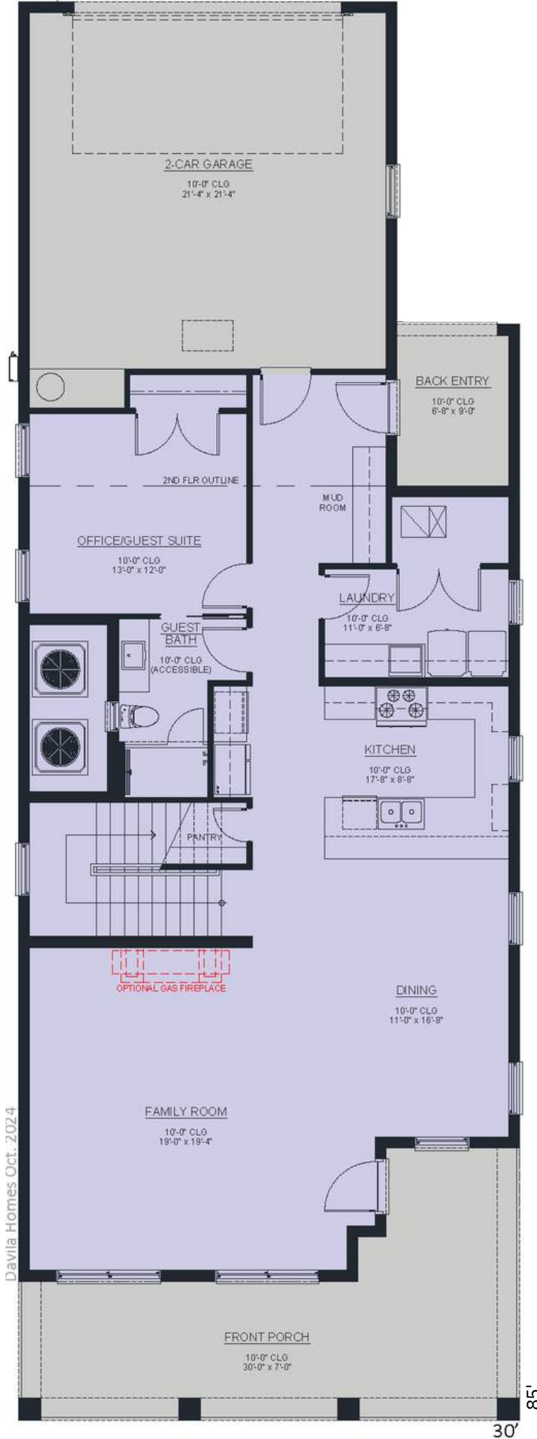
FIRST FLOOR OPTIONAL FIREPLACE
