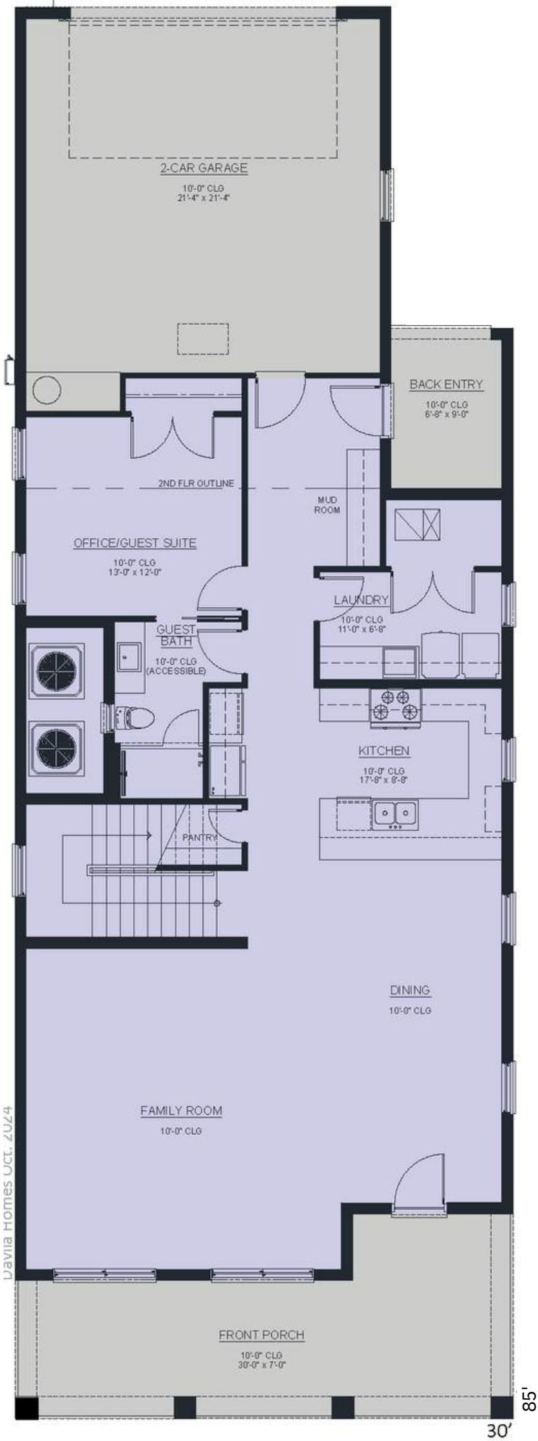
FIRST FLOOR ENTRY SECOND OPTION
